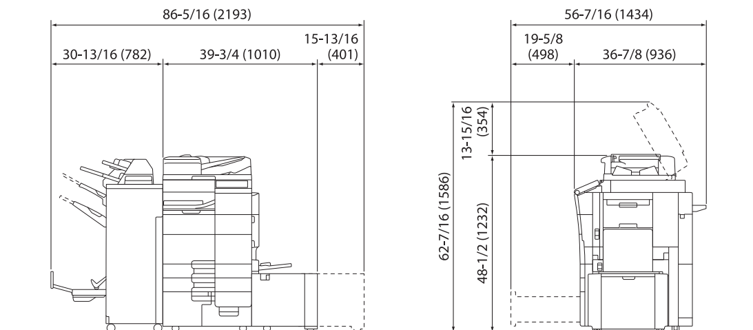
ineo+ 759/659 + FS-537 SD + RU-515 + PI-507 + LU-303
