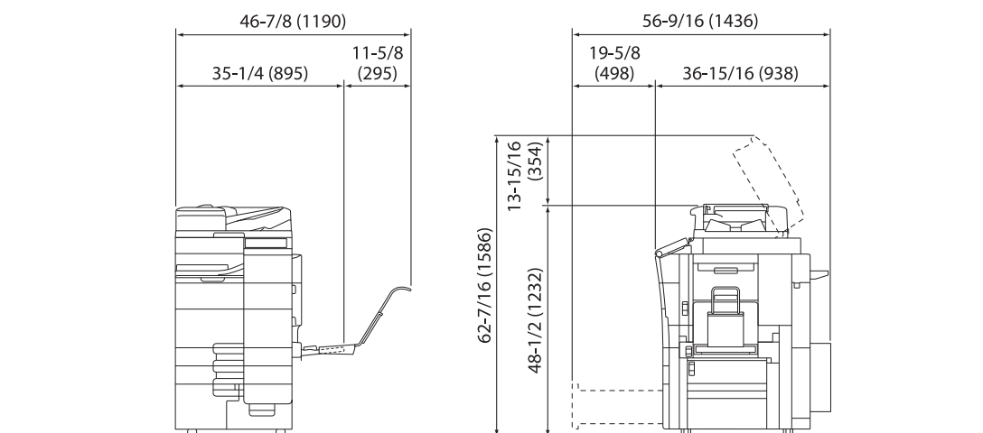
ineo+ 759/659 + MK-715 + CU-102
