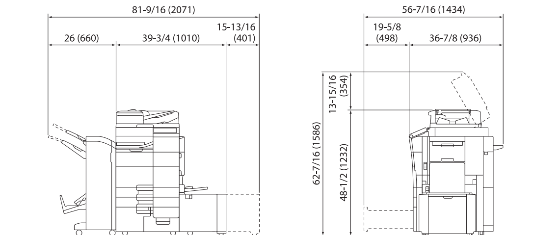
ineo+ 759/659 + FS-536 SD + RU-515 + LU-303
